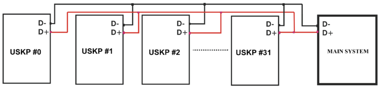
DIAGRAM # 2 DAISY-CHAIN WIRING
